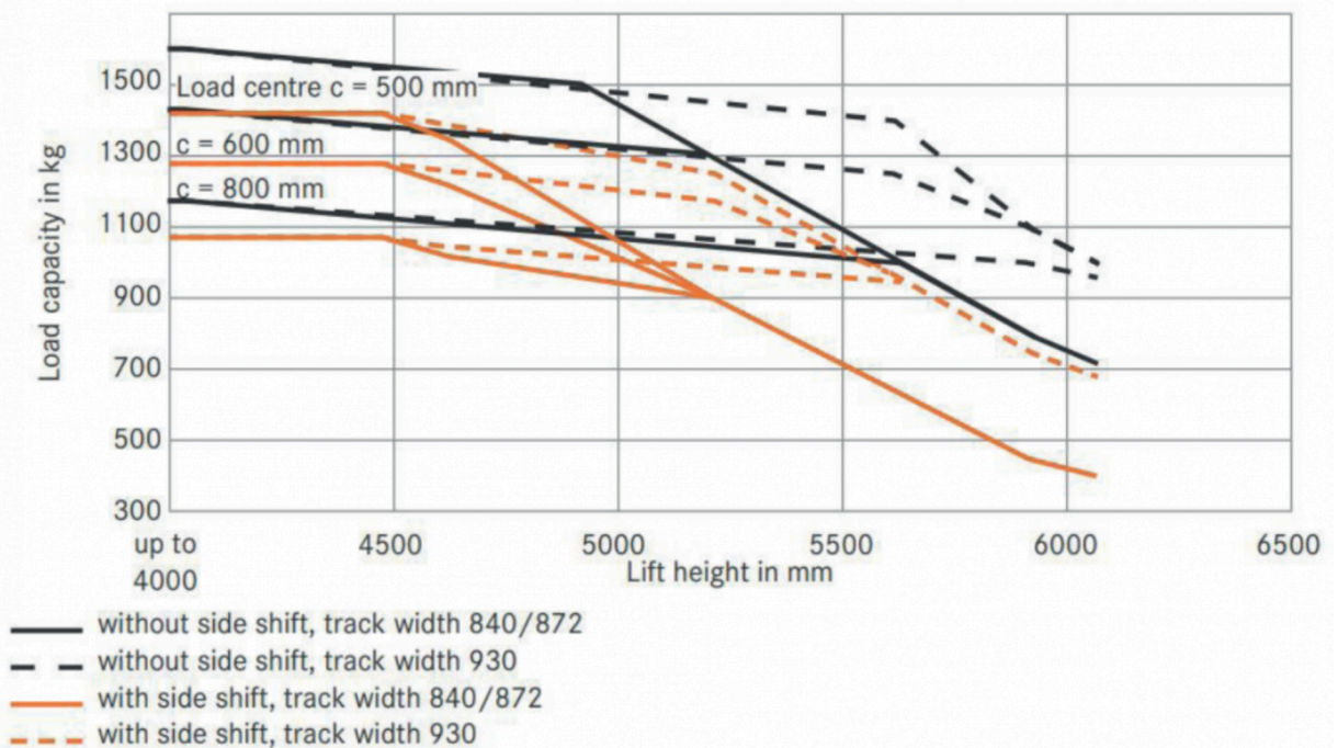
RX 50-16 triplex mast, Superelastic tyres
